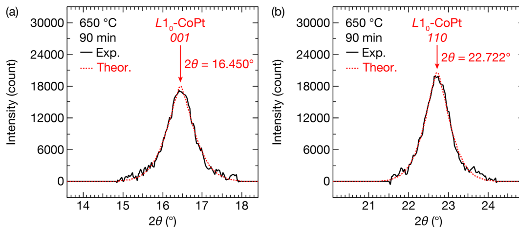
Fig. 3 Intensity– 2\theta 1D GI-XRD profiles of (\text{Co/Pt})_6 nanowires on \text{Si/SiO}_2 substrates after annealing 650^\circ\text{C} for 90 min. Each of the experimental peaks (black curve) of (a) L1_0 -CoPt 001 and (b) L1_0 -CoPt 110 was analyzed by a bell-shaped function after subtracting the remaining background signal. These theoretical curves are plotted as red dotted curves.
