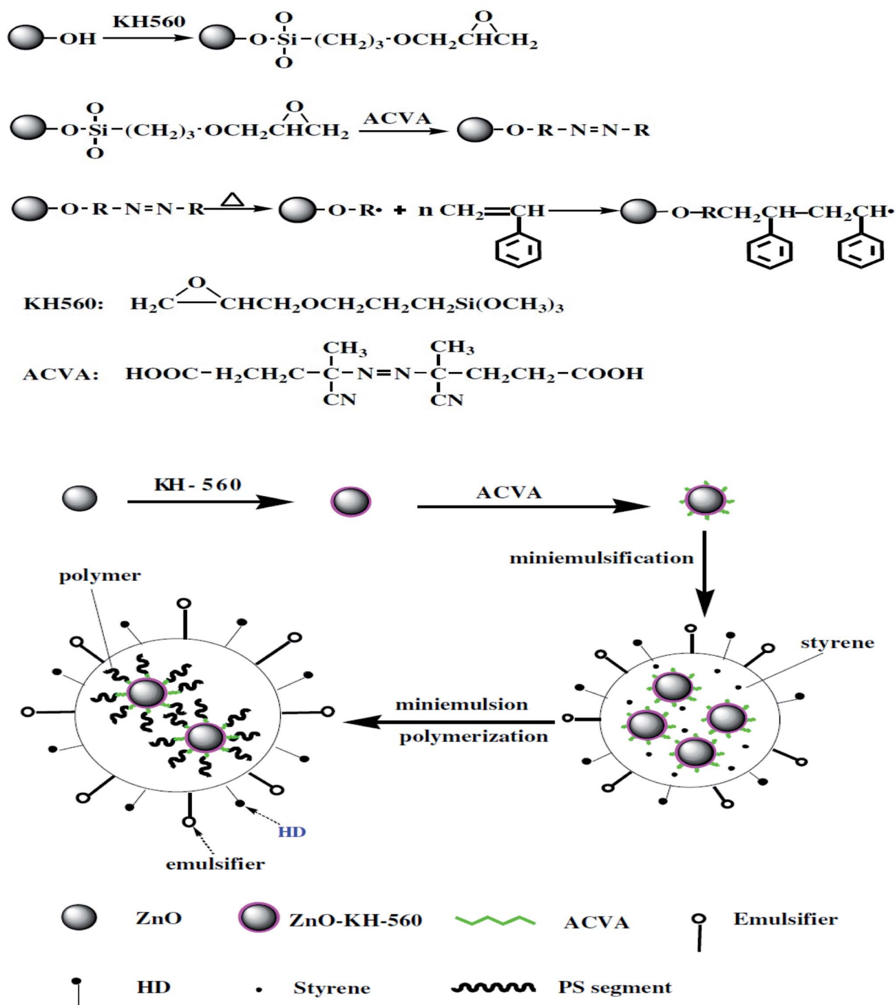
Fig. 5 A schematic diagram showing the synthesis of ZnO/polystyrene nanocomposites by anchoring 4,4'-azobis(4-cyanovaleic acid) (ACVA) onto the surface of ZnO nanoparticles to initiate styrene polymerization (reproduced from ref. 97 with permission from Elsevier).
