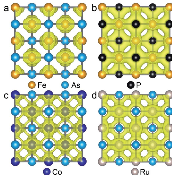
Fig. 4 Isosurface plots of the partial charge density of state 1 in FeAs (a), FeP (b), CoAs (c) and RuAs (d) monolayers with an isosurface value of 0.054 \text{ e } \text{Å}^{-3} .
