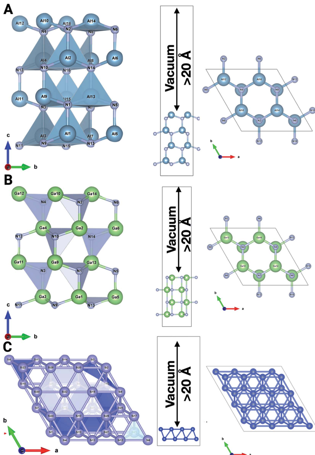
Fig. 1 The system comprising a (3 \times 3 \times 1) supercell for the Si (001) surface, and a (1 \times 1 \times 3) supercell for AlN (001) and GaN (001) pristine surfaces with a vacuum of >20 Å.
