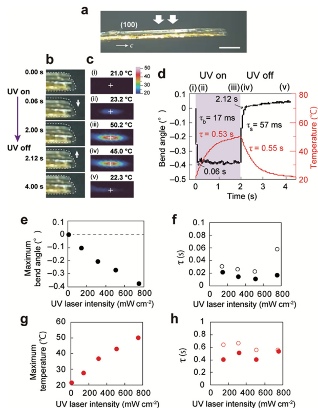
Fig. 4 Bending of a thick enol- 1a crystal ( 2910 \times 331 \times 194 \mu\text{m}^3 ) by the photothermal effect upon UV laser irradiation (Movie S3, ESI † ). (a) Photograph of the crystal (side view). Scale bar: 500 \mu\text{m} . (b and c) Sequential snapshots of the crystal taken in (b) side view using a digital microscope and (c) top view using an infrared thermography camera. (d) Time dependence of the bend angle (black) and maximum surface temperature (red). (e–h) UV laser intensity dependence of the (e) maximum bend angle, (f) time constants for bending (solid circles) and straightening (open circles), (g) maximum top surface temperature, and (h) time constants for temperature increase (solid circles) and decrease (open circles).
