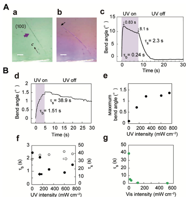
Fig. 3 Bending of thin enol- 1a crystals ((A) 385 \times 30 \times 3.8 \mu\text{m}^3 , Movie S1, (ESI † ) (B) 1980 \times 67.5 \times 31.4 \mu\text{m}^3 , Movie S2, ESI † ) by photoisomerisation upon UV laser irradiation. Photographs of the crystal (a) before and (b) under UV irradiation. Scale bars: 50 \mu\text{m} . (c and d) Time profile of the bend angle. (e and f) UV light intensity dependence of the (e) maximum bend angle and (f) time constants for bending (solid circles) and straightening (open circles). (g) Visible light intensity dependence of the straightening time constant.
