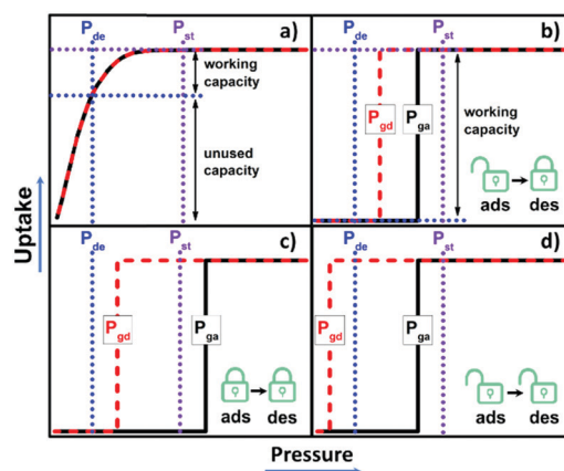
Scheme 1 Comparison of different types of gas sorption isotherms. (a) type I; (b) type F-IV ( P_{de} < P_{gd} < P_{ga} < P_{st} ); (c) type F-IV ( P_{de} < P_{gd} < P_{ga} < P_{st} ) and (d) type F-IV ( P_{gd} < P_{de} < P_{ga} < P_{st} ). Black solid line: adsorption; red dash line: desorption; P_{ga} : gate adsorption pressure; P_{gd} : gate desorption pressure; P_{de} : delivery pressure; P_{st} : storage pressure; ads: adsorption; des: desorption.
