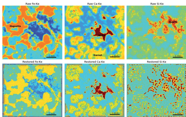
Fig. 9 XRF images of an iron skarn sample.
