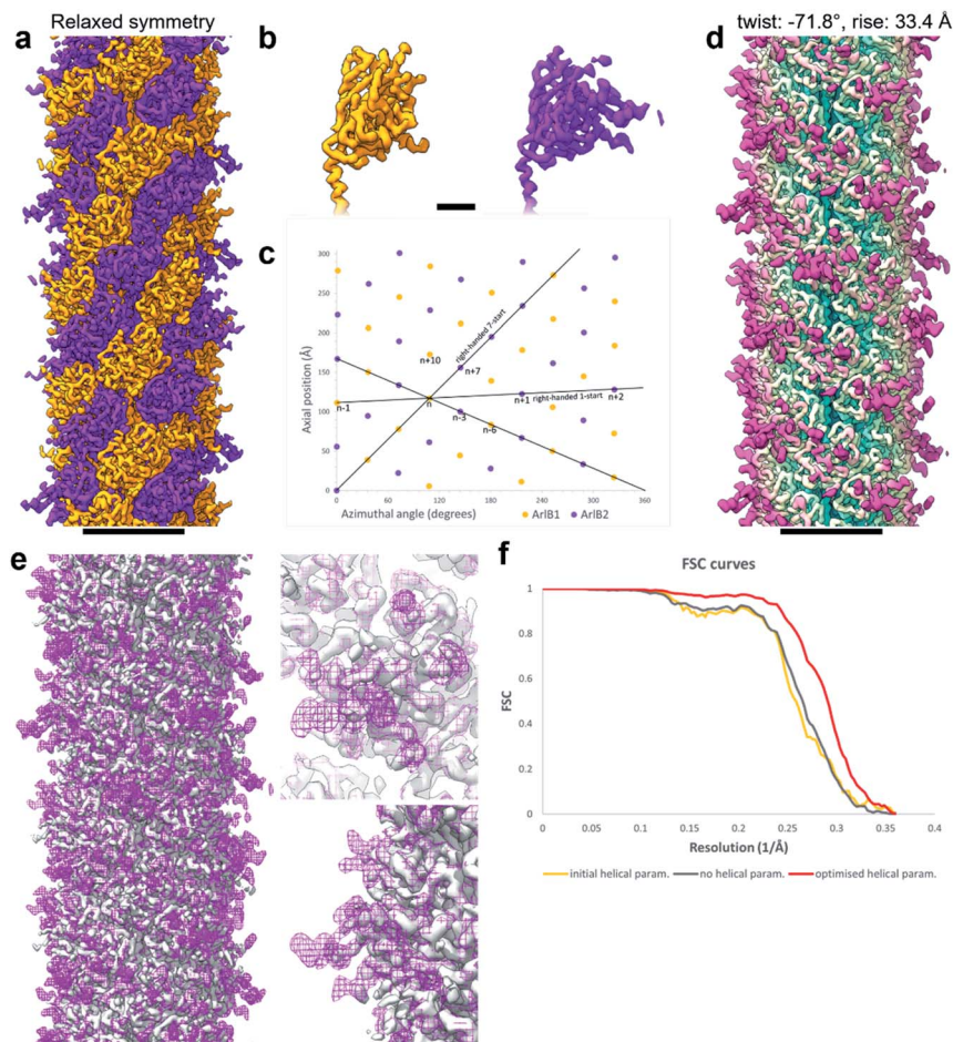
Fig. 3 Refining helical parameters after symmetry relaxation. (a) CryoEM map of the M. villosus archaeellum filament solved with relaxed helical symmetry showing ArlB1 in orange and ArlB2 in purple. (b) Close-up of the head domains of ArlB1 (orange) and ArlB2 (purple). (c) Helical net diagram showing the positions of ArlB1 (orange dots) and ArlB2 (purple dots) in a two-dimensional plot. Solid black lines show various component helices. (d) CryoEM map of the archaeellum filament solved imposing helical symmetry with refined parameters of -71.8^\circ twist and 33.4 \text{ \AA} rise. The map is coloured in petrol blue–light yellow–magenta from the core to the periphery of the filament. (e) Superposition of the cryoEM map obtained relaxing the helical symmetry (solid grey) and cryoEM map obtained applying refined helical parameters (mesh magenta). Two close-ups show the peripheral areas best resolved using the refined helical parameters. (f) Fourier shell correlation curves comparison between the cryoEM maps obtained with initial helical parameters ( 108^\circ twist and 5.5 \text{ \AA} rise; orange), relaxed helical symmetry (grey), refined helical parameters ( -71.8^\circ twist and 33.4 \text{ \AA} rise; red). Scale bar in (a, d, e), 50 \text{ \AA} ; in (b), 10 \text{ \AA} .
