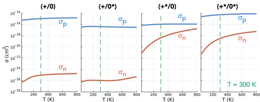
Fig. 6 Electron and hole capture cross-section ( \sigma_n and \sigma_p ) as functions of temperature T for the \text{Te}_i (+*/0^{(*)}) charge transition levels in CdTe. Room temperature ( T = 300 K) denoted by the dashed green line as a guide for typical solar cell operating conditions.
