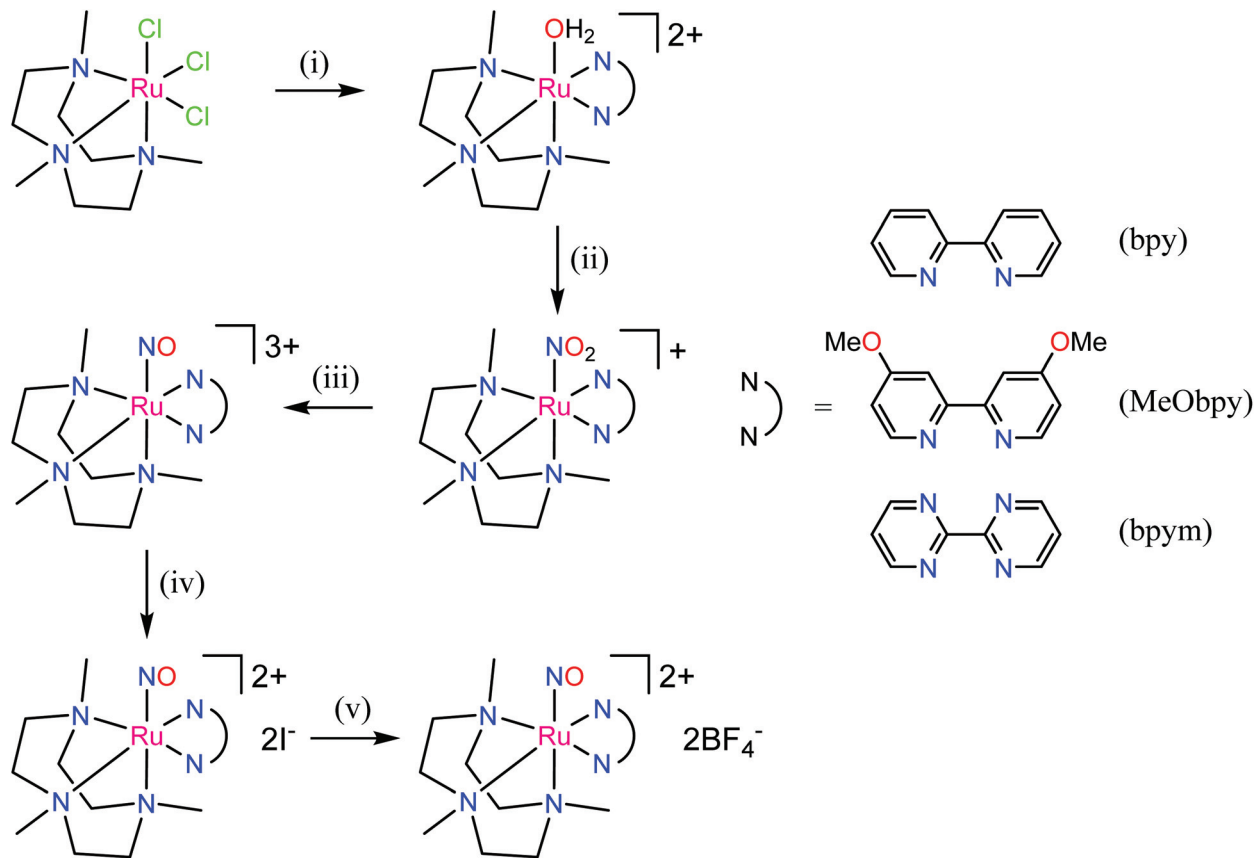
Scheme 3 Synthetic route to \{Ru(NO)\}^7 complexes. Reagents and conditions: (i) bpy, MeObpy or bpym, Zn powder, aqueous solution; (ii) NO_2^- ; (iii) HOF; (iv) acetone, I^- ; (v) Dowex 22 ( BF_4^- ), then lyophilization.
