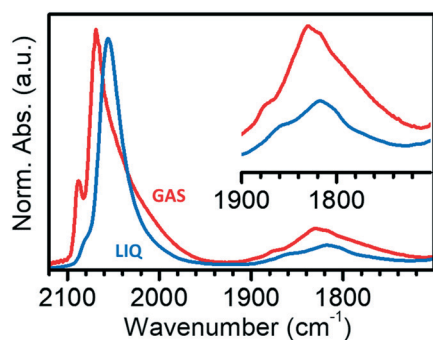
Fig. 4 IR spectra of CO adsorbed at room temperature on \text{Pt}/\text{Al}_2\text{O}_3 activated and reduced at 70 °C in gas-phase (GAS) and in liquid-phase (LIQ) in the \nu(\text{CO}) region. The inset reports a magnification of the 1900–1700 \text{cm}^{-1} region of multi-coordinated carbonyls. Spectra GAS and LIQ were arbitrarily normalized to the intensity of band L2.
