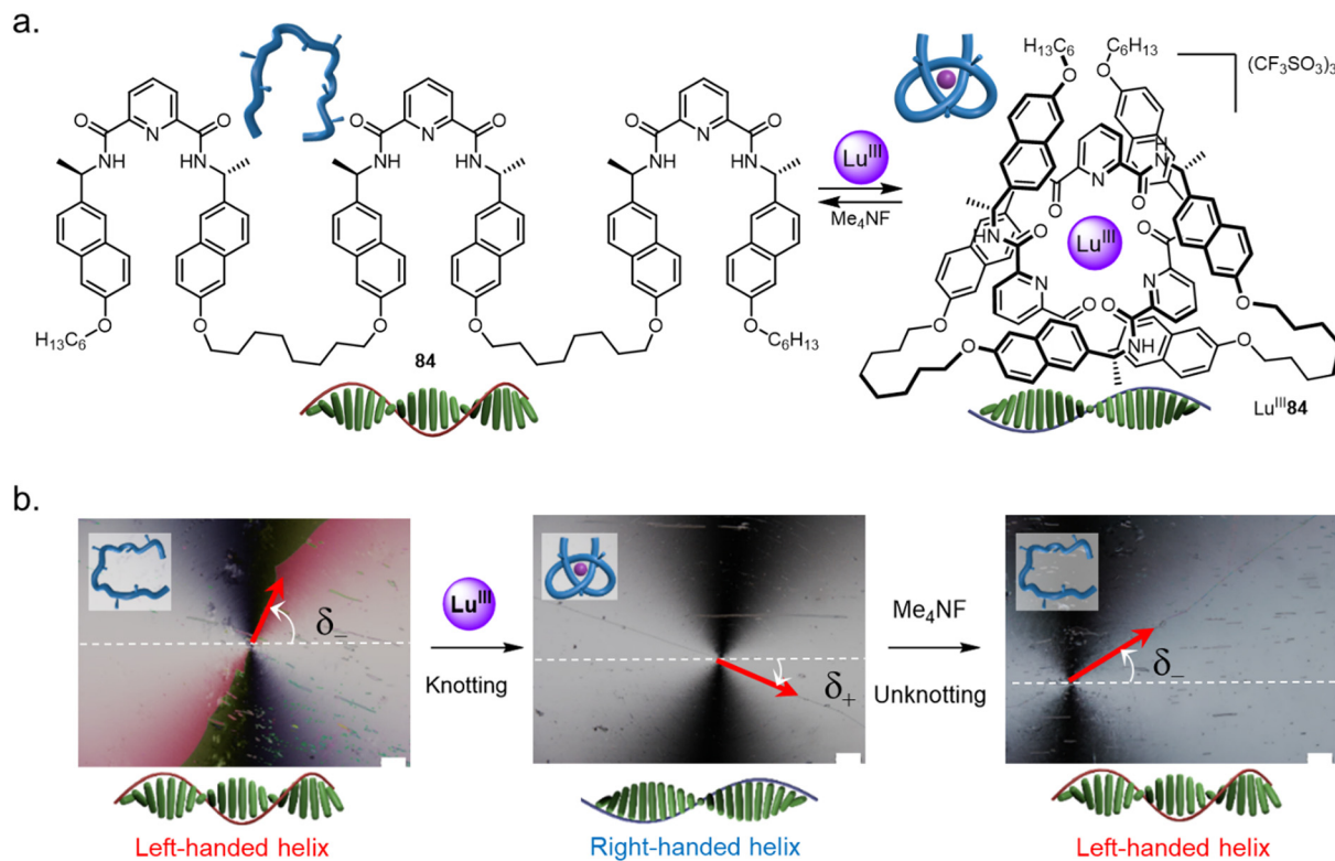
Fig. 34 Tying a molecular knot inverts chirality expression in liquid crystals. (a) Left-handed helical liquid crystal organization with homochiral strand 84 as a dopant, while right-handed organization occurs with the corresponding knot \text{Lu}^{\text{III}}\mathbf{84} . (b) The knot can be tied and untied in situ to reversibly invert the chiral expression within the liquid crystal, as evidenced by polarized optical microscopy photographs of \theta -cell disclination lines. 137 Reworked from ref. 137 with permission from the authors, copyright 2020.
