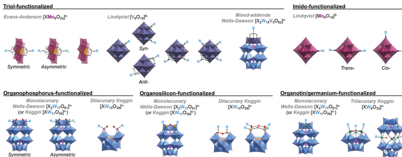
Fig. 1 Library of the most commonly studied hybrid POM platforms and functionalisation strategies. Colour code: \{Mo_6O_6\} = purple polyhedra, \{Mo_6O_6\} = orange polyhedra, \{VO_6\} = grey/blue polyhedra, \{WO_6\} = blue polyhedra, \{PO_4\} = purple tetrahedra, \{SiO_4\} = orange tetrahedra, O = red, N = blue, P = pink, Si = orange, Sn = green.
