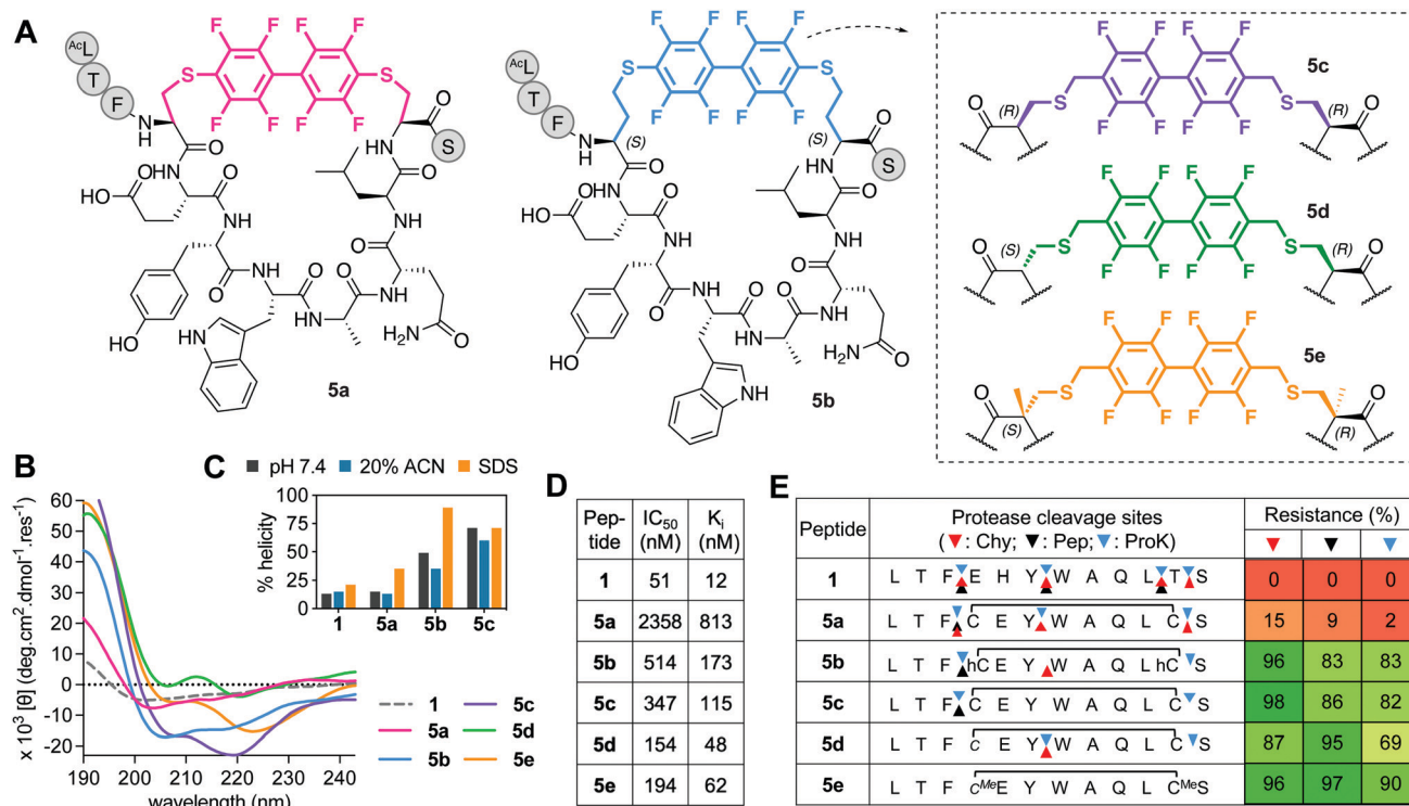
Fig. 5 A. Structures of perfluorobiphenyl ( i \rightarrow i + 7 )-crosslinked peptides 5a–e . B. CD spectra for 5a–e vs. 1 (50 \mu\text{M} ) in 10 mM phosphate buffer (pH 7.4, 22 ^{\circ}\text{C} ). C. Percent helicity calculated from CD spectra ( \theta_{220} ) in 10 mM phosphate buffer, 20% ACN or 20 mM SDS buffer ( 5d,e not helical). D. \text{IC}_{50} = mean peptide concentration to inhibit 50% binding of fluorescent 1-FITC (10 nM) to hDM2 (25 nM) measured by FP. \text{pIC}_{50} \pm \text{SEM} values are reported in Fig. S1 (ESI ^{\dagger} ). Binding affinity ( K_i ) calculated from \text{IC}_{50} values. E. Heatmap indicating percent peptide intact after 2 h incubation with chymotrypsin (Chy), pepsin (Pep) or proteinase K (ProK) at 22 ^{\circ}\text{C} , pH 8 or 2 (Pep only), measured by LCMS. Arrows point to the respective cleavage sites as revealed by LCMS analysis of the cleaved fragments.
