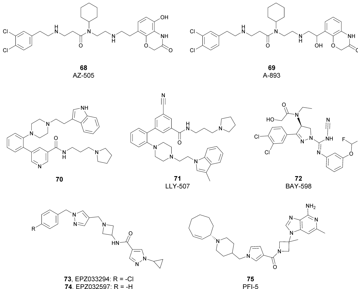
Fig. 18 SMYD2 inhibitors.
