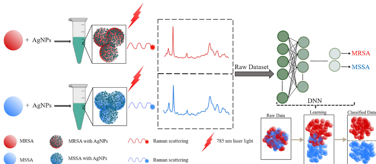
Fig. 7 General workflow of deep learning-based spectral data analysis for the discrimination of MRSA and MSSA. The image is reprinted from Ciloglu et al. , 100 Copyright (2021), with permission from Springer Nature.
