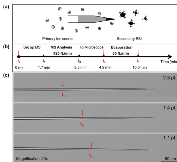
Fig. 1 Conducting and measuring femto flow electrospray ionization mass spectrometry. (a) Scheme of the relay ESI setup. The sample solution (black) in the secondary emitter was ionized by electrospray triggered by charges from a primary ion source. In the secondary emitter, a hexane layer (grey) reduced sample evaporation. (b) Timeline of a typical experiment that collects both mass spectra and flow rate data. (c) Microscopy images of the emitter at three time points. Red arrows indicate the phase boundary between the aqueous sample (right) and hexane (left).
