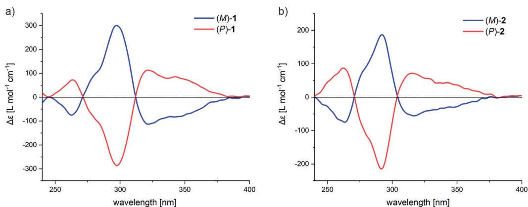
Fig. 6 Circular dichroism spectra of (a) ( P )- 1 (red) and ( M )- 1 (blue), (b) ( P )- 2 (red) and ( M )- 2 (blue) in CH 2 Cl 2 ( c \sim 10^{-6} M). Absolute configuration was assigned according to exciton chirality method, DFT calculations and X-ray crystallography.
