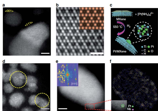
Fig. 3 TEM characterization of 1 wt% \text{Pt}/\text{MXene} catalysts. (a) Representative HAADF-STEM image of the 1% \text{Pt}/\text{Ti}_3\text{C}_2\text{T}_x catalyst. (b) (111) surface of \text{Pt}_3\text{Ti} NPs. The inset shows a simulated STEM image of the \text{Pt}_3\text{Ti}(111) surface. The simulated image is in good agreement with the experimental results. (c) Schematic illustration of reactive metal-support interactions in \text{Pt}/\text{MXene} catalysts and the structure of L12-ordered intermetallic \text{Pt}_3\text{Ti} . (d) Representative HAADF STEM image of the 1% \text{Pt}/\text{Nb}_2\text{CT}_x catalyst. (e) \text{Pt} – \text{Nb} NPs viewed along [111] , the inset shows the FFT pattern of the NPs. (f) IFFT pattern of the NPs in (e). The inset shows the enlarged image showing the superlattice of the NPs. Scale bars: (a, d, e) 2 nm, and (b) 500 pm. Reprinted from ref. 27 (open access).
