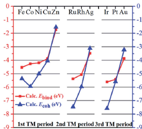
Fig. 6 Calculated binding energy ( E_\text{bind} , red squares, left y-axis) and the corresponding bulk cohesive energy ( E_\text{coh} , blue triangles, right y-axis) for \text{M}/\text{Mo}_2\text{CO}_{2-\delta} ( \text{M} = \text{Fe}, \text{Co}, \text{Ni}, \text{Cu}, \text{Zn}, \text{Ru}, \text{Rh}, \text{Ag}, \text{Ir}, \text{Pt}, \text{and Au} ). Reprinted with permission from ref. 44, copyright 2019 John Wiley and Sons.
