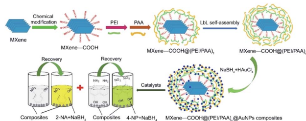
Fig. 8 Graphic design of synthesis and catalysis of \text{MXene-COOH} @ (\text{PEI} / \text{PAA})_n @ \text{AuNP} nanocomposites. Reproduced with permission from ref. 65, copyright 2018 Elsevier.
