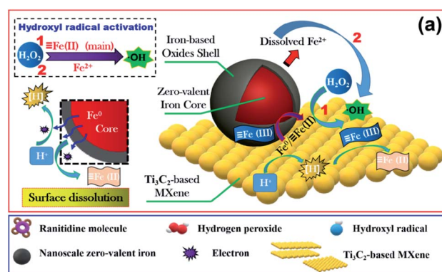
Fig. 14 Schematic of the mechanism of ranitidine catalytic degradation by the ( n\text{ZVI} )@ \text{Ti}_3\text{C}_2 /H 2 O 2 system. Reprinted with permission from ref. 78, copyright 2021 Elsevier.
