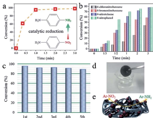
Fig. 10 Catalytic performance of the Pd/ \text{Ti}_3\text{C}_2\text{Tx} /graphene hydrogel for (a) hydrogenation of 4-NA; (b) hydrogenation of other nitro-derivatives; (c) cycling performance for 4-NA dehydrogenation; (d) picture of the catalyst after the hydrogenation reaction; (e) schematic illustration of the catalytic dehydrogenation reaction. Reproduced with permission from ref. 69, copyright 2020 Elsevier.
