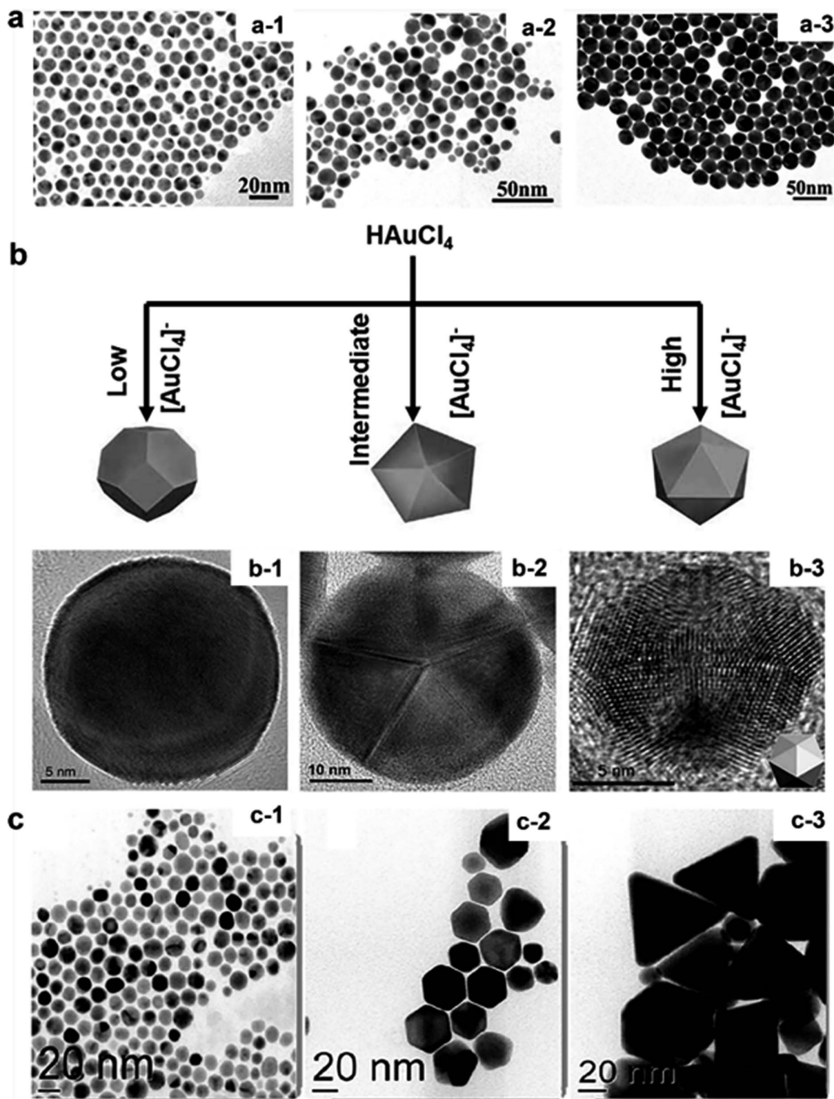
Fig. 2 (a) Transmission electron microscope (TEM) images of Au nanoparticles (NPs) prepared at different temperatures: (a-1) 75 °C; (a-2) 95 °C; and (a-3) 115 °C. Reproduced with permission. 65 Copyright 2008, American Chemical Society. (b) Crystallinity tunable synthesis of Au NP nanoparticles. (b-1) High resolution TEM (HRTEM) images of single-crystalline Au NPs; (b-2) round decahedral Au multiply twinned particle; (b-3) icosahedral Au multiply twinned particle. Reproduced with permission. 66 Copyright 2010, Wiley-VCH. (c) TEM images of Au NPs formed using (c-1) dioleamide only, (c-2) a 1 : 1 molar ratio of dioleamide and oleic acid, and (c-3) a 1 : 2 molar ratio of dioleamide and oleic acid. Reproduced with permission. 38 Copyright 2010, American Chemical Society.
