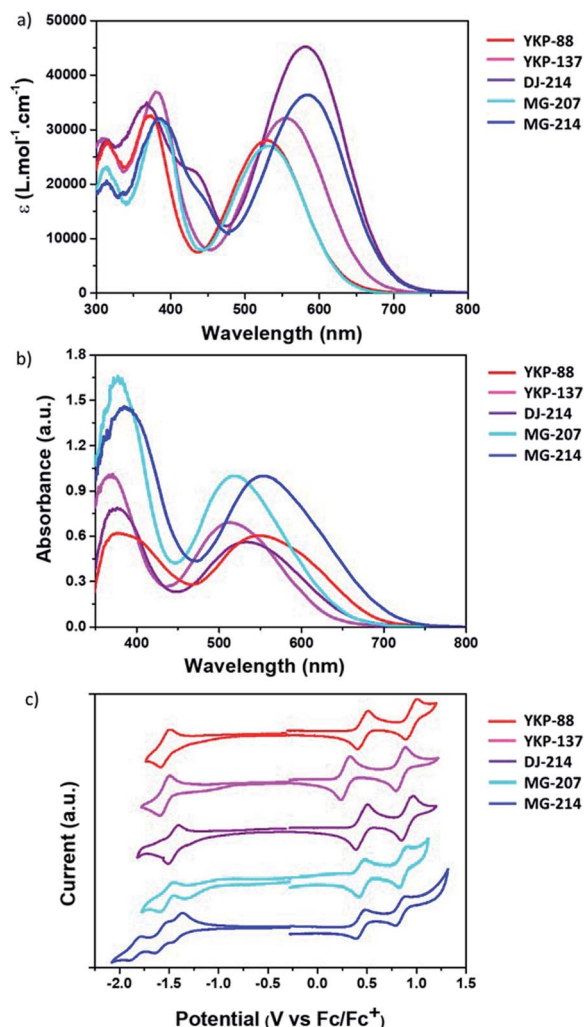
Fig. 3 (a) Absorption spectra registered (a) in Dichloromethane solution, ( 10^{-5} M, 25 °C), (b) on 2 \mu\text{m} -thick mesoporous \text{TiO}_2 electrodes, for compounds YKP-88 (red line), YKP-137 (magenta line), DJ-214 (violet line) MG-207 (cyan line) and MG-214 (blue line) (c) cyclic voltammetry traces in solution for each compound (deoxygenated dichloromethane, 10^{-3} M, 25 °C, voltage scan 200 \text{mV s}^{-1} ).
