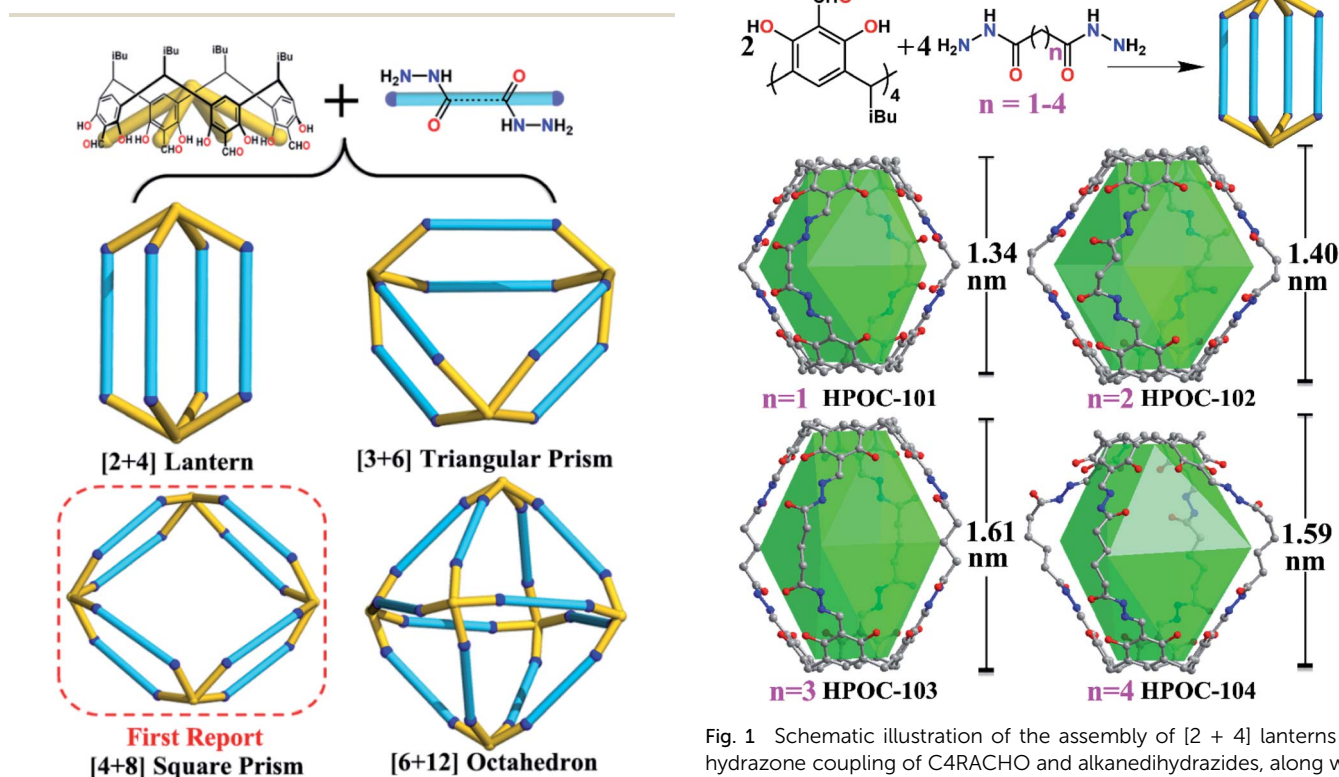
Scheme 1 Self-assembly of organic cages constructed from the tetraformyl C4RACHO cavitand and dihydrazide linkers.
