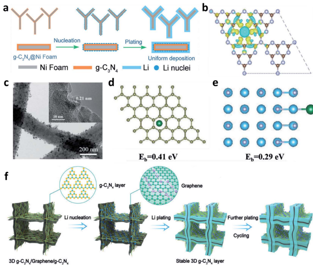
Fig. 13 (a) Schematic illustration of the preparation of a \text{g-C}_3\text{N}_4 layer on Ni foam and its effects towards regulating \text{Li}^+ uniform deposition; (b) charge distribution of the \text{g-C}_3\text{N}_4 layer revealing that N atoms have higher electron density and can absorb positively charged \text{Li}^+ ; 134 reproduced with permission. Copyright 2019, John Wiley and Sons. (c) TEM images of the TiN-decorated 3D carbon fibre; (d) optimized geometries for calculating the binding energy of a Li atom adsorbed on TiN, and (e) the corresponding charge density difference; 136 reproduced with permission. Copyright 2019, John Wiley and Sons. (f) Schematic illustration of the Li deposition on the 3D \text{g-C}_3\text{N}_4/\text{G}/\text{g-C}_3\text{N}_4 electrode. 137 Reproduced with permission. Copyright 2021, John Wiley and Sons.
