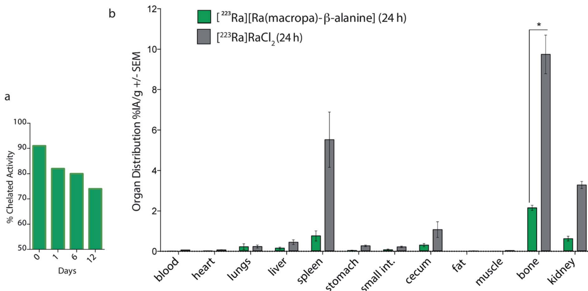
Fig. 6 In vitro and in vivo evaluation of [^{223}\text{Ra}][\text{Ra}(\text{macropa-}\beta\text{-alanine})] . (a) Stability of [^{223}\text{Ra}][\text{Ra}(\text{macropa-}\beta\text{-alanine})] over the course of 12 days in human serum at 37 \text{ }^\circ\text{C} . (b) Organ distribution of [^{223}\text{Ra}][\text{Ra}(\text{macropa-}\beta\text{-alanine})] at 24 h p.i. Significant differences in osseous ( *p < 0.005 ), splenic, and renal uptake were observed in comparison to the control [^{223}\text{Ra}]\text{RaCl}_2 .
