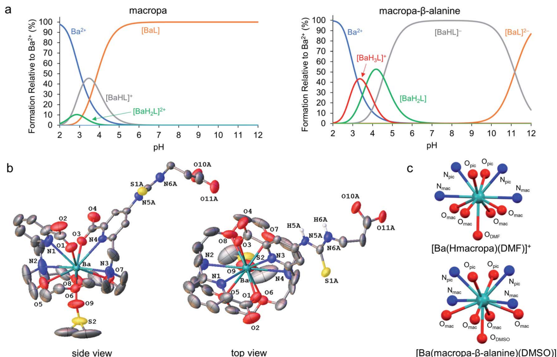
Fig. 5 Alkaline earth metal complexes of macropa- \beta -alanine. (a) Species distribution diagrams of macropa (left) and macropa- \beta -alanine (right) in the presence of Ba^{2+} at [Ba^{2+}]_{\text{tot}} = [L]_{\text{tot}} = 1.0 \text{ mM} , I = 0.1 \text{ M KCl} , and 25 \text{ }^\circ\text{C} . (b) X-ray crystal structure of [Ba(\text{macropa-}\beta\text{-alanine})(\text{DMSO})] . Ellipsoids are drawn at the 50% probability level. Nonacidic hydrogen atoms are omitted for clarity. A full discussion of the crystallographic disorder of the structure is provided in the ESI.† (c) Comparison of the immediate coordination sphere of the Ba^{2+} center in the crystal structures of [Ba(\text{Hmacropa})(\text{DMF})]^+ and [Ba(\text{macropa-}\beta\text{-alanine})(\text{DMSO})] .
