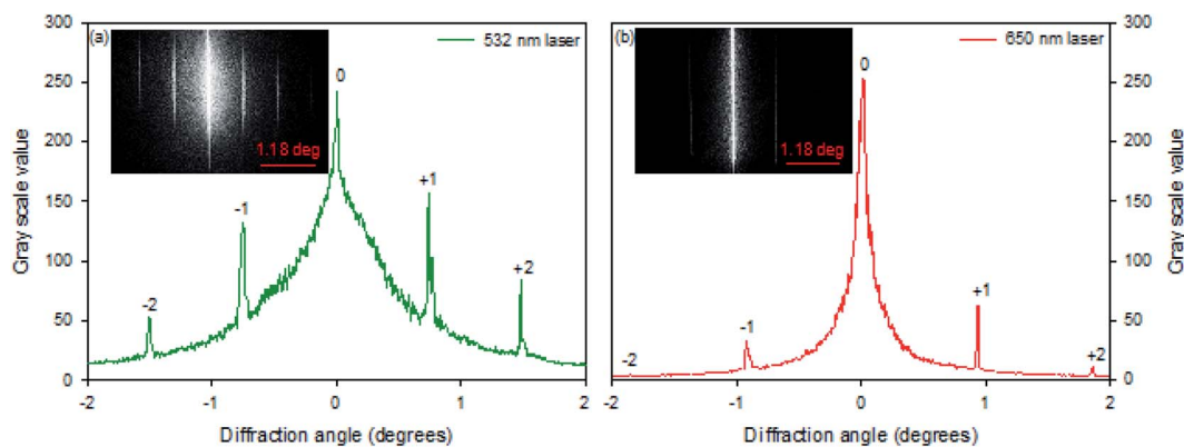
Fig. 3 Diffraction patterns 40.13 \mu\text{m} pitch hydrogel gratings illuminated with lasers of peak wavelength of (a) 532 nm and (b) 650 nm.
