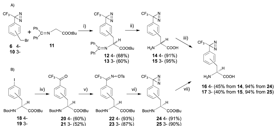
Fig. 4 Synthesis of (3- and 4-trifluoromethyldiazirinyl)-D-phenylalanine derivatives. (i) CsOH, Bu 4 NBr, CH 2 Cl 2 , rt, 12 h, (ii) TFA, rt, 2 h, (iii) L-amino acid oxidase, pH 7.0, 37 °C, 12 h, (iv) (1) MeLi, (2) tBuLi, (3) CF 3 CO 2 Et, toluene, −78 °C, 12 h, (v) (1) NH 2 OH·HCl, pyridine, 70 °C, 1.5 h, (2) TsCl, TEA, acetone, rt, 1 h, (vi) NH 3 (l), ether, 80 °C, 9 h, (vii) TFA, rt, 8 h.
