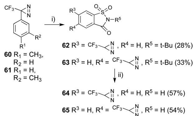
Fig. 9 Synthesis of 5- or 6-trifluoromethyldiazirine saccharin derivatives. (i) (1) ClSO 3 H, TiCl 4 , −20 °C, 1 h, then rt, 4 h, (2) t -BuNH 2 , CH 2 Cl 2 , 0 °C, 2 h, then rt, 22 h, (3) H 5 IO 6 , CrO 3 , Ac 2 O, CH 3 CN, 0 °C, 0.5 h, then rt, 48 h, (ii) CF 3 COOH, reflux, 24 h.
