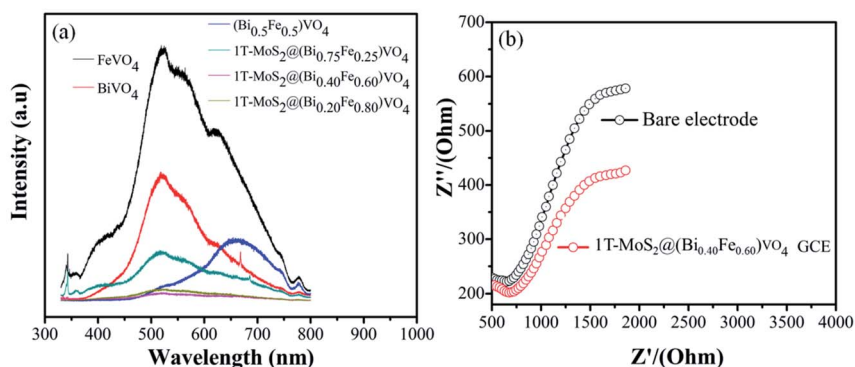
Fig. 7 (a) PL spectra (excited at 325 nm) of composites at different concentrations and (b) EIS Nyquist plots of the bare and as-modified \text{1T-MoS}_2@(\text{Bi}_{0.40}\text{Fe}_{0.60})\text{VO}_4 nanocomposite GCE samples.
