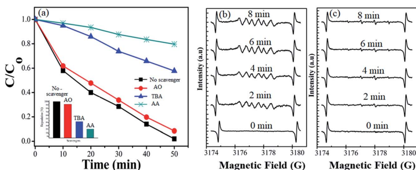
Fig. 8 (a) Effects of different radical scavengers on CV degradation over \text{1T-MoS}_2@(\text{Bi}_{0.40}\text{Fe}_{0.60})\text{VO}_4 under visible light irradiation. (b) DMPO spin trapping EPR spectra for \text{DMPO}\cdot\text{O}_2^- and (c) \text{DMPO}\cdot\text{OH}^- under visible light over \text{1T-MoS}_2@(\text{Bi}_{0.40}\text{Fe}_{0.60})\text{VO}_4 photocatalyst.
