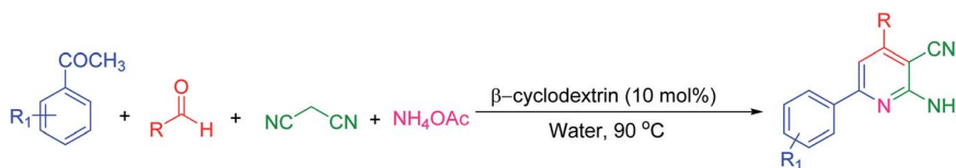
Scheme 1 One-pot four-component synthesis of 2-amino-4,6-disubstituted nicotinonitriles.
