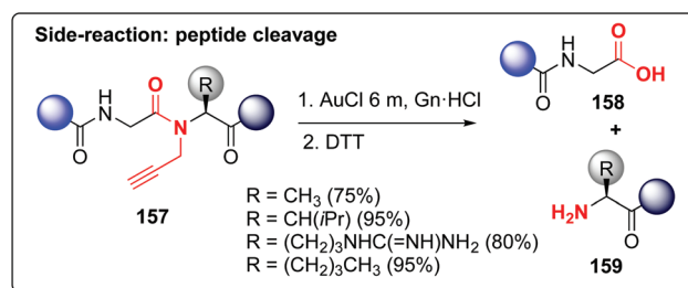
Scheme 37 N-Removable protecting groups by Brik et al. 118
