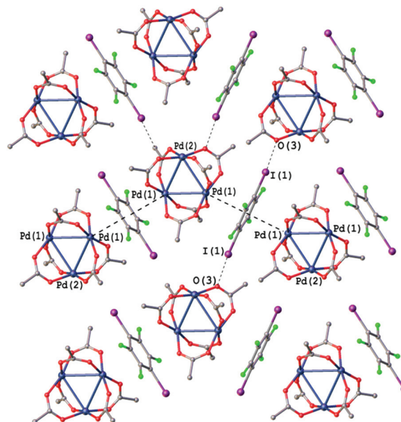
Fig. 8 Crystal structure diagram of [Pd 3 ](1,4-IFB). Selected distances (Å): I(1)...O(3) 3.399, Pd...([Pd 3 ]) centroid 3.349. Short I...O contacts and PdO 4 ... \pi interactions are clearly seen in the Hirshfeld surface map (Fig. S5†).
