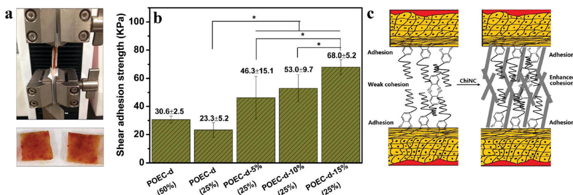
Fig. 14 (a) Image of lap-shear measurement set-up (top) and two pieces of adhered porcine skins after tensile breaking; (b) the lap-shear adhesion strength using wet porcine as the adherent. POEC-d (50%) and POEC-d (25%) are the catechol-based adhesive with aqueous weight concentration in water in brackets. POEC-d-5%, POEC-d-10%, and POEC-d-15% are the POEC-d adhesives with 5, 10 and 15% (w/w) ChNCs with respect to POEC-d. (c) Proposed mechanism of heightened adhesion caused by addition of ChNC. (* p < 0.05 ). Adapted from ref. 229.
