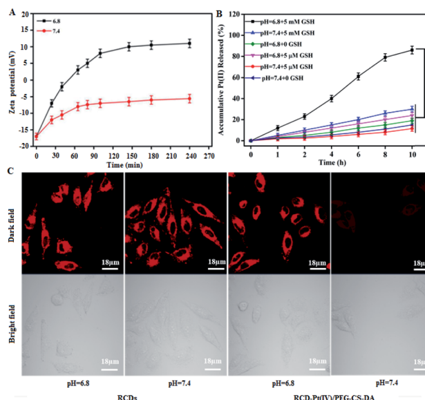
Fig. 2 (A) Zeta potential of RCD-Pt(IV)/PEG-CS-DA under different conditions. (B) The effect of pH value and GSH concentration on the RCD-Pt(IV)/PEG-CS-DA releasing Pt(IV). (C) Laser confocal fluorescence imaging of T24 cells after incubation (excitation: 405 nm; emission: 680 nm). The error bar represents the standard deviation ( n = 3 ). The statistical analysis was performed using the Student's t -test method, *** p < 0.001 .
