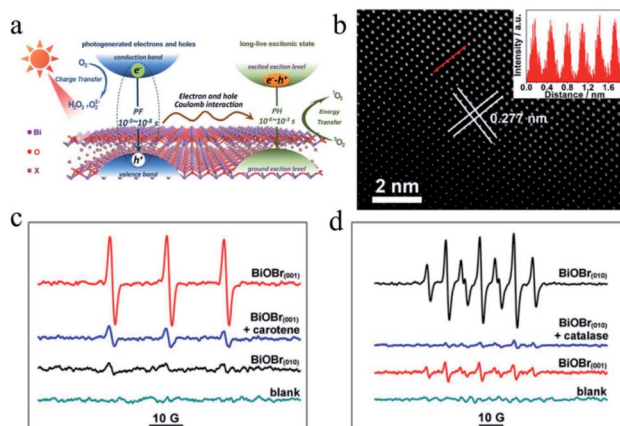
Fig. 10 (a) Schematic illustration of optical relaxation excitation processes presented in confined layered structure systems, where PH and PF are phosphorescence and prompt fluorescence, respectively. (b) Atomic-resolution scanning transmission electron microscopy (STEM) image of \text{BiOBr}(001) . (c and d) Electron spin resonance (ESR) spectra. Reproduced with permission from ref. 115 Copyright 2017, the American Chemical Society.
