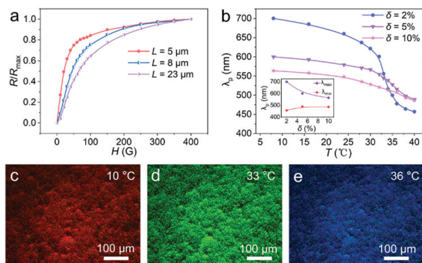
Fig. 5 The influence of L and \delta on the optical properties of the \text{Fe}_3\text{O}_4 @PVP@PNIPAM flexible PNCs. (a) Plots showing the magnetic field strength responsive optical properties of the flexible PNCs with different L values. (b) Plots showing the temperature-responsive optical properties of the flexible PNCs with different \delta values. The inset in (b) shows the maximum and minimum diffraction wavelengths of the flexible PNCs with different \delta values. (c–e) Dark-field optical microscopy images of the flexible PNCs with \delta = 2\% at different temperatures.
