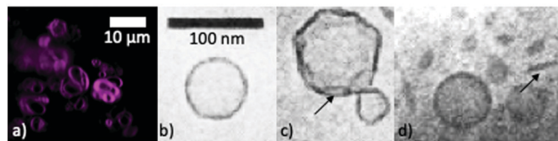
Fig. 13 (a) Confocal microscopy image of a luminescent dye embedded in the lipid bilayer of giant DMPC vesicles. Figure adapted from ref. 39. CryoTEM images of (b) extruded DMPC ( T_m = 23 °C) vesicles vitrified from 40 °C, (c) extruded DPPC ( T_m = 41 °C) vesicles vitrified from 25 °C, and (d) sonicated DLPA ( T_m = 31 °C) vesicles vitrified from 18 °C. Adapted with permission from M. Andersson, L. Hammarström and K. Edwards, J. Phys. Chem. , 1995, 99 , 14531–14538. Copyright (1995) American Chemical Society. 34
