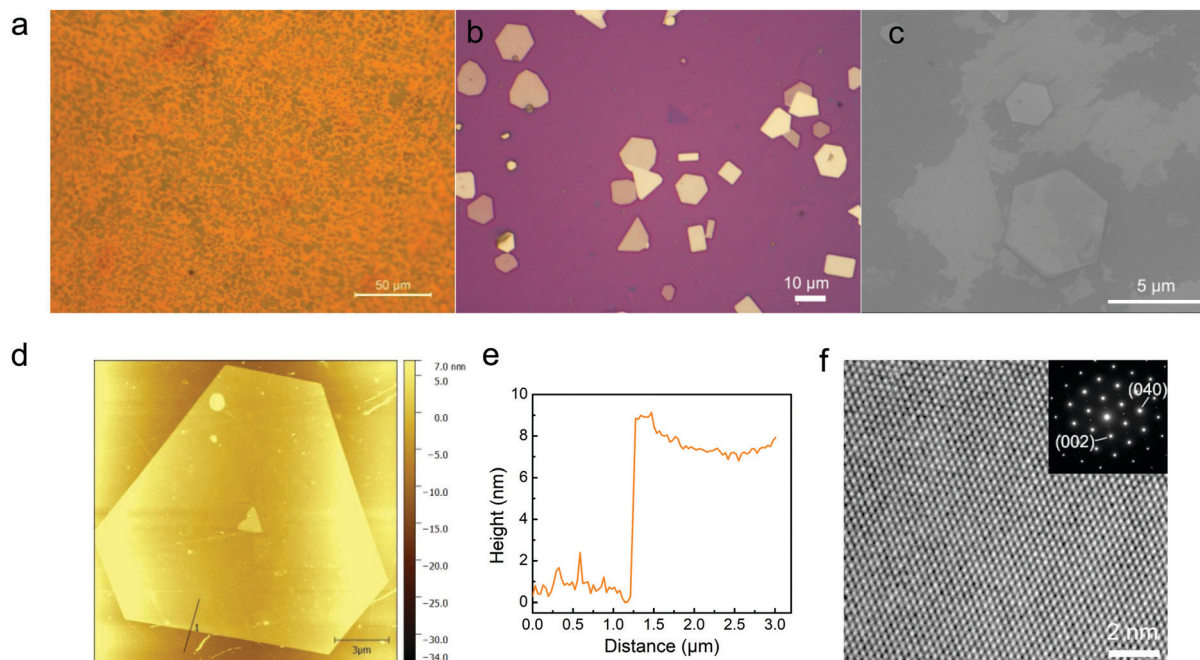
Fig. 1 (a) Optical image of graphene– \text{Mo}_2\text{C} grown on a Cu foil. (b) Optical image of graphene– \text{Mo}_2\text{C} after transferred to the Si/SiO 2 substrate. (c) SEM image of the graphene– \text{Mo}_2\text{C} heterostructure. (d) AFM topography of the graphene– \text{Mo}_2\text{C} heterostructure. (e) AFM cross-sectional profile along the black line in (d). (f) HRTEM image of \text{Mo}_2\text{C} showing the atomic structure. The inset shows the SAED result.
