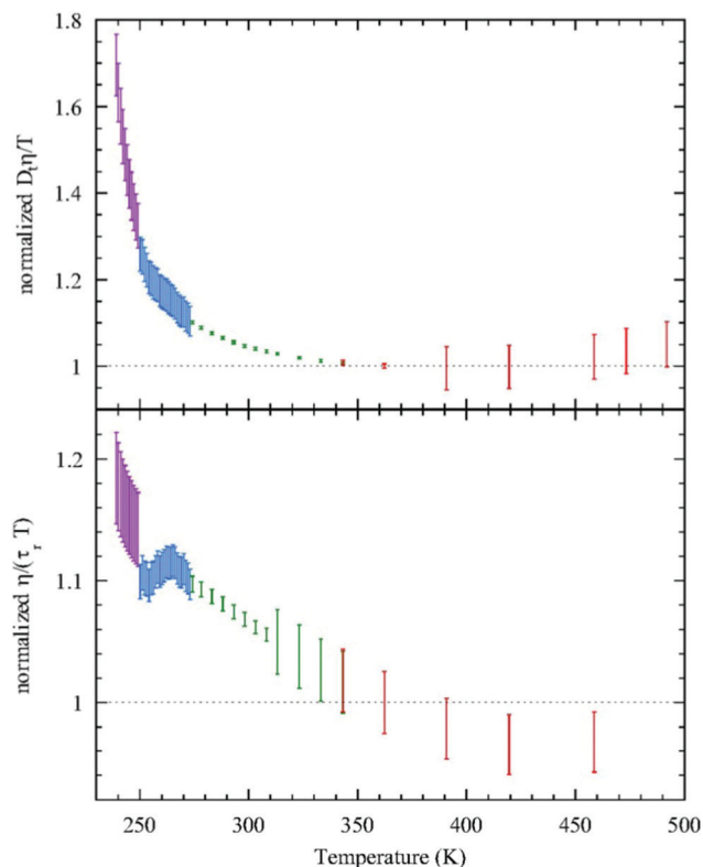
Fig. 4 Test of the SER (upper panel) and SEDR (lower panel). D\eta/T (upper) and \eta/(\tau_T T) (lower) were plotted as a function of temperature. Here, the diffusion coefficient was denoted by D , while the molecular rotation time was denoted by \tau_T . The data were further normalized by their value at 362.25 K. The SER and SEDR relations would thus correspond to the horizontal dotted lines. SER and SEDR hold at high temperatures, but they are violated by around 70% and 18% at low temperatures, respectively. Reprinted with permission from ref. 54.
