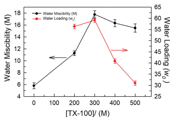
Fig. 2 Plots depicting water miscibility ( M ) and water loading ( w_0 ) within the TX-100/TBAC-DA system for different concentrations of TX-100.
