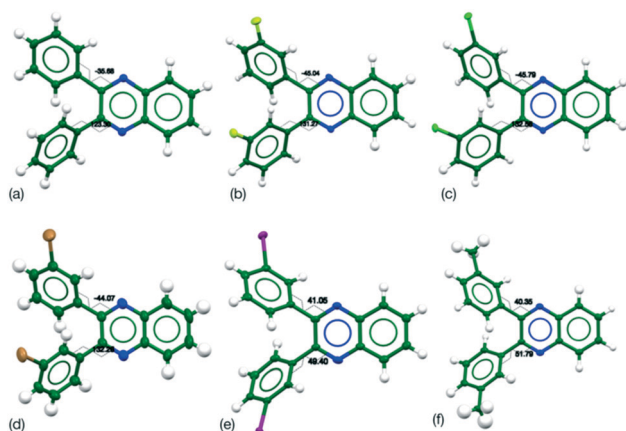
Fig. 1 Molecular conformations in the crystal structures of Q3,3'X 2 (a) X = H, (b) X = F, (c) X = Cl, (d) X = Br, (e) X = I, (f) X = Me. Carbon atoms are displayed as dark green spheres, nitrogen as blue, fluorine as yellow, chlorine as light green, bromine as brown, iodine as purple and hydrogen as white. Thermal ellipsoids are shown for 50% probability levels for all.
