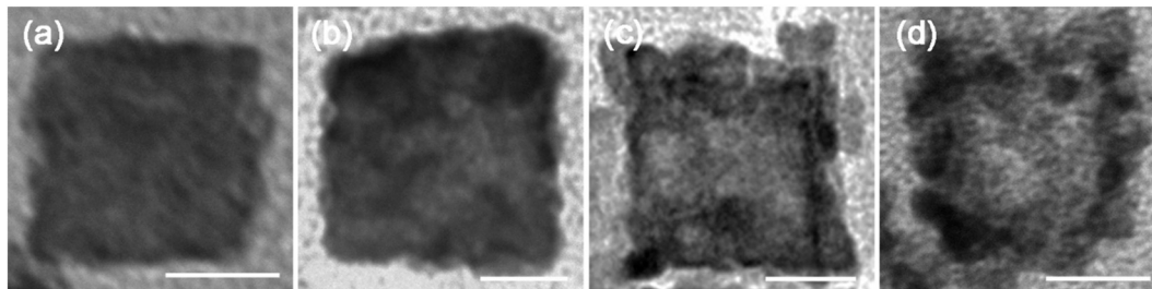
Fig. 5 TEM images of the products obtained at different reaction times: (a) 10 min, (b) 50 min, (c) 120 min and (d) 160 min. All the scale bars are 100 nm.
