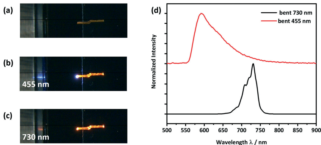
Fig. 8 Optical microscope images of a) the bent crystal placed on a silicon wafer with a 3 \mu\text{m} thick \text{SiO}_2 layer, (b) showing light with a wavelength of 455 nm being coupled at the left end of the crystal and (c) showing light with a wavelength of 730 nm being coupled at the left end of the crystal; (d) detected PL-spectra at the right end of the crystal.
