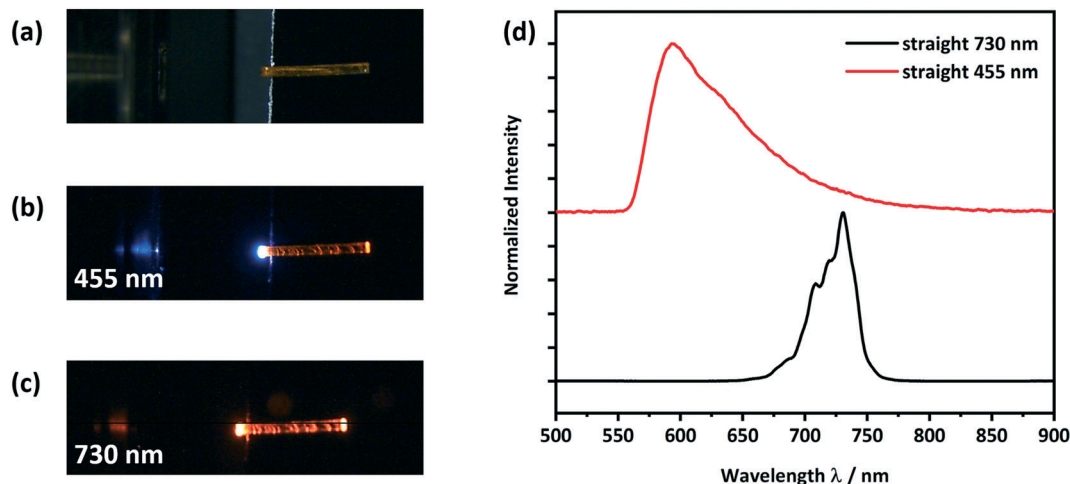
Fig. 7 Optical microscope images of a) a form II straight crystal placed on a silicon wafer with a 3 \mu\text{m} thick \text{SiO}_2 layer as shown in Scheme S1, † b) showing light with a wavelength of 455 nm being coupled at the left end of the crystal and c) showing light with a wavelength of 730 nm being coupled at the left end of the crystal; d) detected PL spectra at the right end of the crystal. The spectra of the LED light sources, PLE and PL are given in Fig. S11 and S12. †
