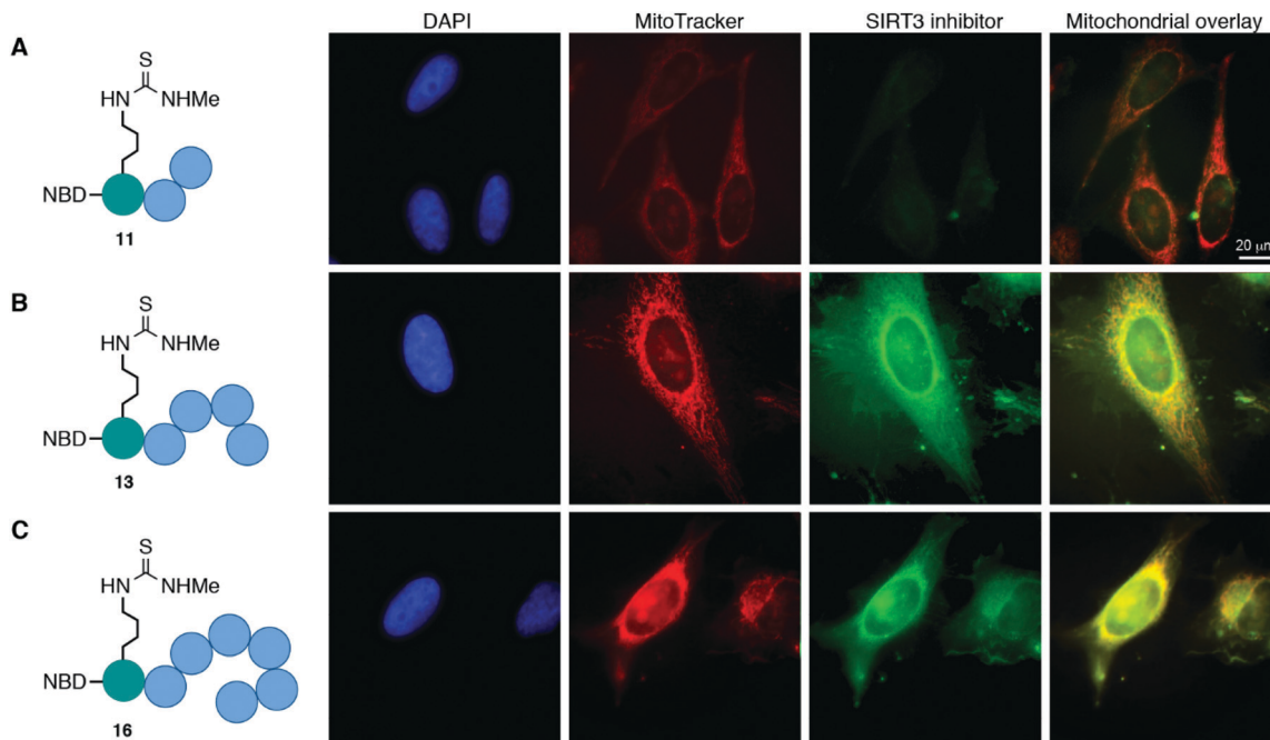
Fig. 3 Mitochondrial targeting of fluorophore labeled inhibitors in HeLa cells, determined by co-staining with MitoTracker™. (A) NBD-labeled trimer ( 11 ); pearson correlation coefficient ( r ) = -0.66 . (B) NBD-labeled pentamer ( 13 ); pearson correlation coefficient ( r ) = 0.59 . (C) NBD-labeled heptamer ( 16 ); pearson correlation coefficient ( r ) = 0.46 .
