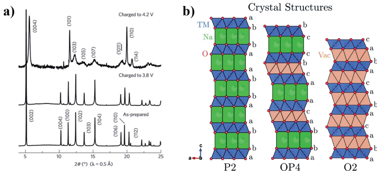
Fig. 3 (a) XRD patterns showing the formation of the OP4-type phase when P2-Na x Fe 1/2 Mn 1/2 O 2 is charged to 4.2 V. (b) Projections of the P2, OP4 and O2 type crystal structures perpendicular to the stacking axis, highlighting the different stacking sequences. Reproduced from ref. 37 under a CC BY 3.0 licence.
