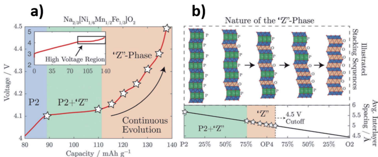
Fig. 4 (a) Voltage profile of Na 2/3 [Ni 1/6 Mn 1/2 Fe 1/3 ]O 2 highlighting the regions in which the “Z” phase forms. (b) Schematic illustration depicting the “Z” phase as a continuously changing intergrowth structure between P2 and O2. Reproduced from ref. 40 under a CC BY 3.0 licence.
