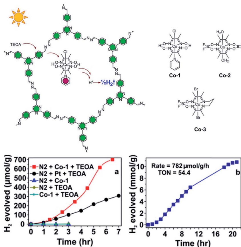
Fig. 8 Structures of the N 2 -COF and the Co-catalysts and their photocatalytic hydrogen evolution performance under AM 1.5 light irradiation. Adapted with the permission of ref. 61. American Chemical Society, Copyright 2017.
