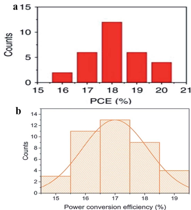
Fig. 22 (a) Histogram of perovskite solar cell efficiencies based on \text{MAPbI}_3\text{:F4TCNQ} films (with 0.03 wt% F4TCNQ). Reproduced by permission ref. 145, Copyright 2018 Springer Nature. (b) Histogram of 40 devices based on \text{MA}_{0.6}\text{FA}_{0.38}\text{Cs}_{0.02}\text{PbI}_{2.975}\text{Br}_{0.025} : 5 mol% MAcl perovskite. Reproduced by permission ref. 146, Copyright 2017 Wiley-VCH Verlag GmbH & Co. KGaA, Weinheim.
