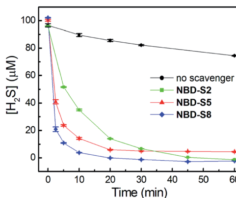
Fig. 5 \text{H}_2\text{S} -scavenging curves of NBD amines or no scavenger in PBS buffer ( \text{pH} 7.4 ) at 25 °C. Three scavengers ( NBD-S2 , NBD-S5 , and NBD-S8 , 110 \mu\text{M} ) were added to \text{H}_2\text{S} solutions (100 \mu\text{M} ). The \text{H}_2\text{S} concentrations were measured using MBA. The results are expressed as mean \pm S.D. ( n = 3 ).
