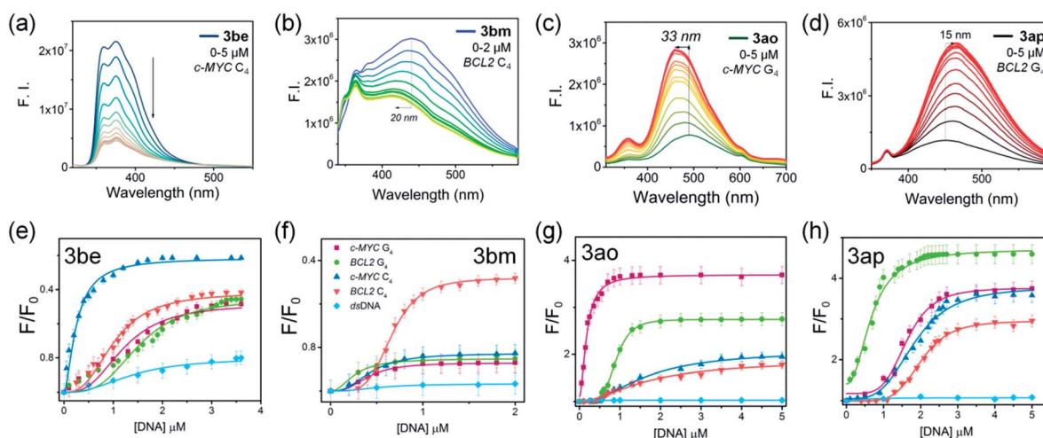
Fig. 8 (a–d) Fluorescence spectroscopic titrations of lead ligands (1 \mu M) with c -MYC C_4 , BCL2 C_4 , c -MYC G_4 and BCL2 G_4 DNA. (e–h) Fluorescence response curves of 3be , 3bm , 3ao and 3ap with incremental addition of c -MYC C_4 (blue), BCL2 C_4 (orange), c -MYC G_4 (purple), BCL2 G_4 (green) and dsDNA (light blue).
