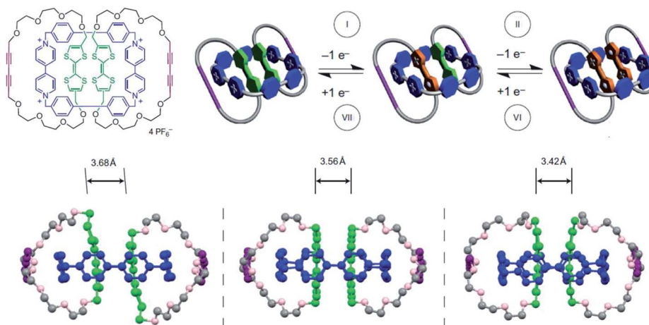
Fig. 17 The chemical structure of the [3]catenanes and their stepwise oxidation. The single crystal structure of (TTF)_2 , (TTF)_2^{++} and (TTF^{+})_2 containing [3]catenanes. Reproduced from ref. 80 with permission from Nature Publishing Group, Copyright 2010.
