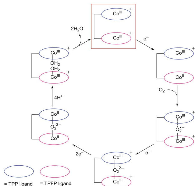
Fig. 6 Proposed catalytic cycle for the ORR with 1. Complex 1 will be instantly oxidized to the Co III Co III oxidation state on the electrode upon applying large positive potentials, and this 2e - oxidized species (highlighted with a red box) is the real starting catalyst.
