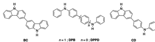
Chart 1 Ditungic secondary amines.
